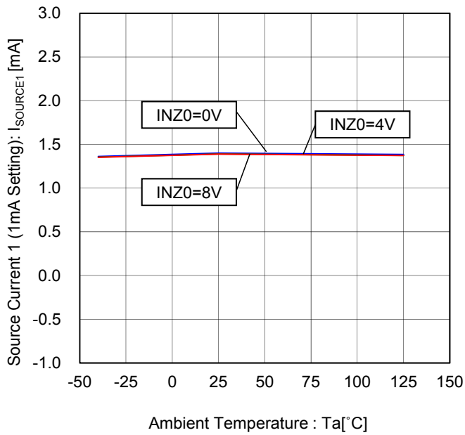
Figure 33. Source Current 1 (1mA Setting) vs Ambient Temperature
