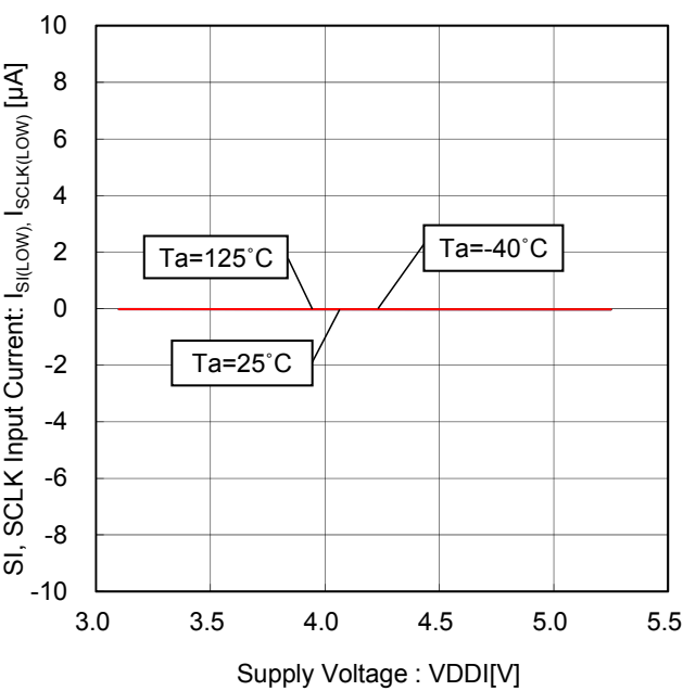
Figure 88. SI, SCLK Input Current vs Supply Voltage (SI, SCLK=0V)
