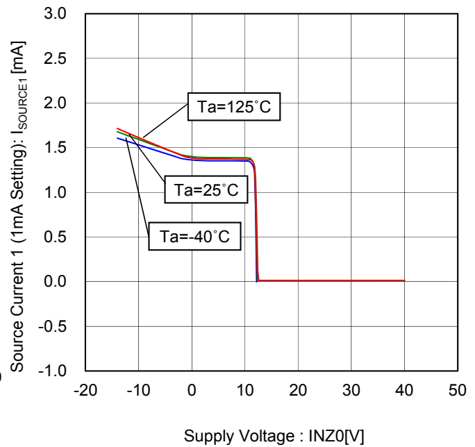
Figure 34. Source Current 1 (1mA Setting) vs Supply Voltage
