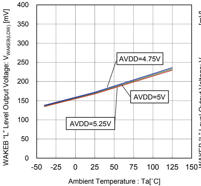
Figure 105. WAKEB "L" Level Output Voltage vs Ambient Temperature (WAKEB=1.0mA)
