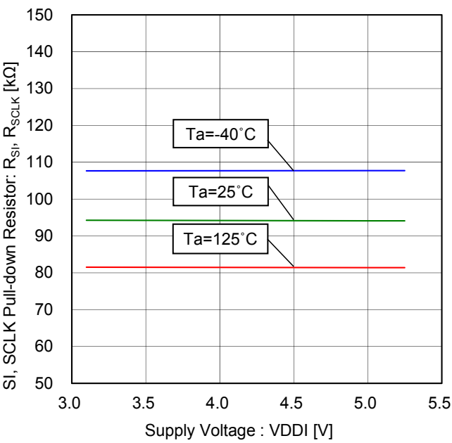
Figure 86. SI, SCLK Pull-down Resistor vs Supply Voltage
