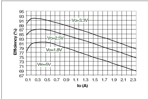
Figure 35. Efficiency vs. output current - V_{IN} = 5\text{ V}
