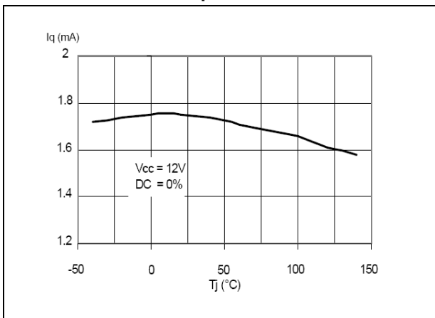
Figure 31. Quiescent current vs. junction temperature
