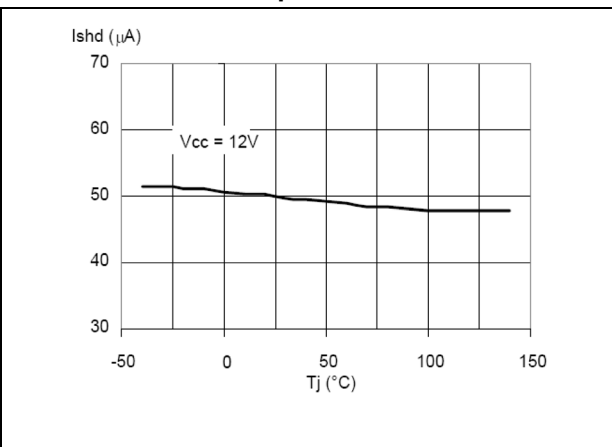
Figure 32. Shutdown current vs. junction temperature
