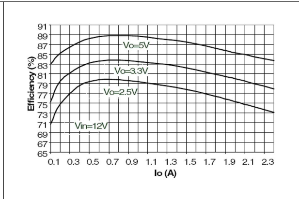
Figure 36. Efficiency vs. output current - V_{IN} = 12\text{ V}
