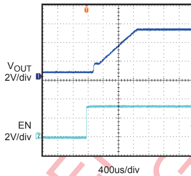
Turn on Delay and Rise Time with 1uF Load, no Cdv/dt C_{OUT} = 1\mu F, \text{no load}
