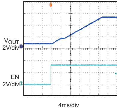
Turn on Delay and Rise Time with 1uF Load C_{OUT} = 1\mu F, \text{no load}
