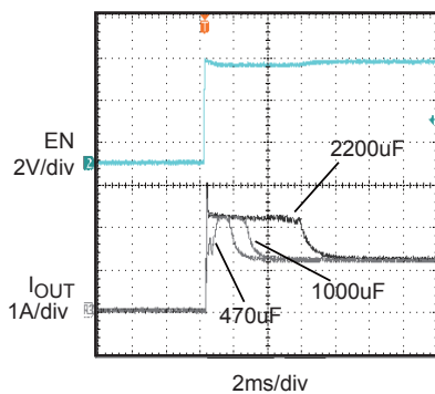
Inrush Current with Different Load Capacitance R_{LOAD} = 3.9\Omega, \text{no } C_{dv/dt}, \text{EN floating}
