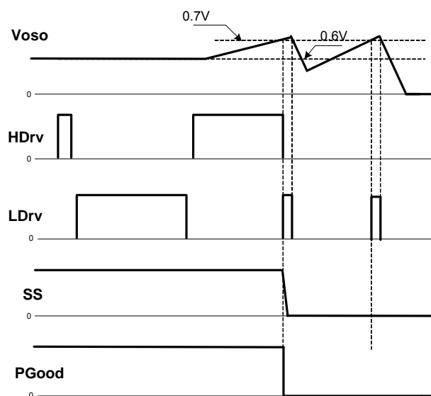
Figure 12b: iP1837 Signal Timing for OVP
