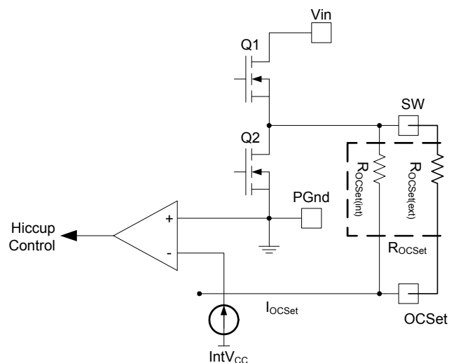
Figure 11: Connection of over-current sensing resistor
