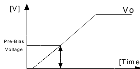
Figure 8: Pre-Bias startup
