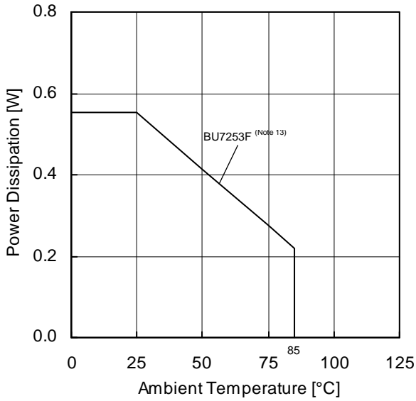
(e) BU7253F
