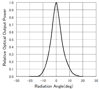
DIRECTIVITY
