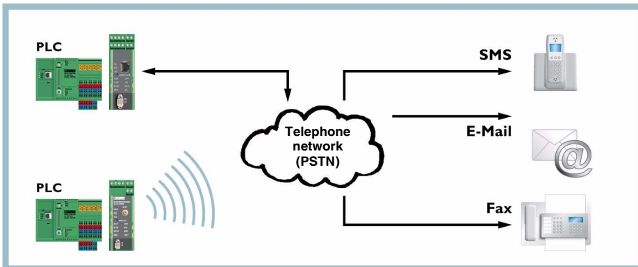
Figure 3 Alarm generation
