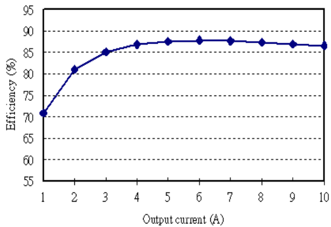
Figure 3: Converter efficiency vs. output current (1.8V output voltage, 12V input)
