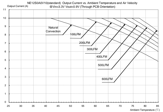
Figure 31: Output current vs. ambient temperature and air velocity @ Vin=3.3V, Vout=0.9V (Through PCB Orientation)
