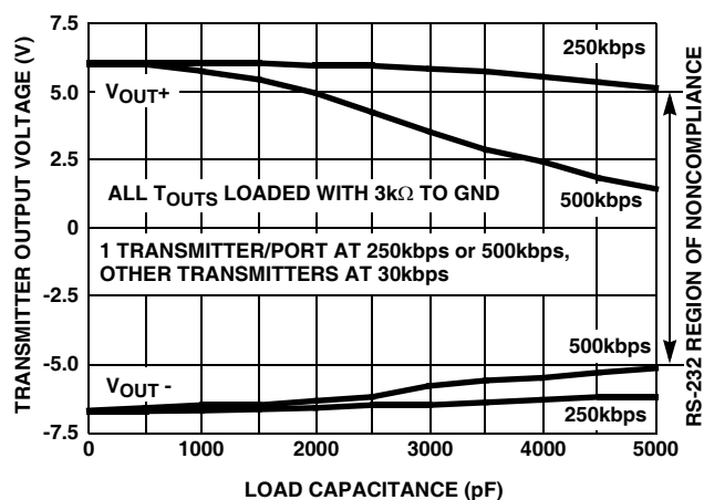
FIGURE 42. RS-232, TRANSMITTER OUTPUT VOLTAGE vs LOAD CAPACITANCE
