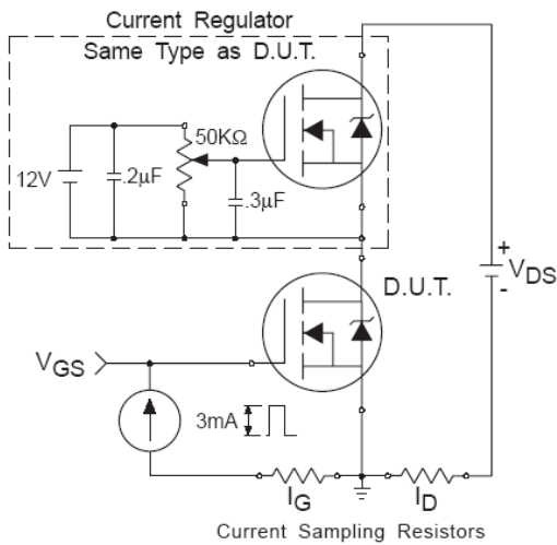
Fig 9b. Gate Charge Test Circuit
