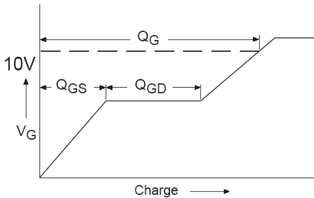
Fig 9a. Basic Gate Charge Waveform
