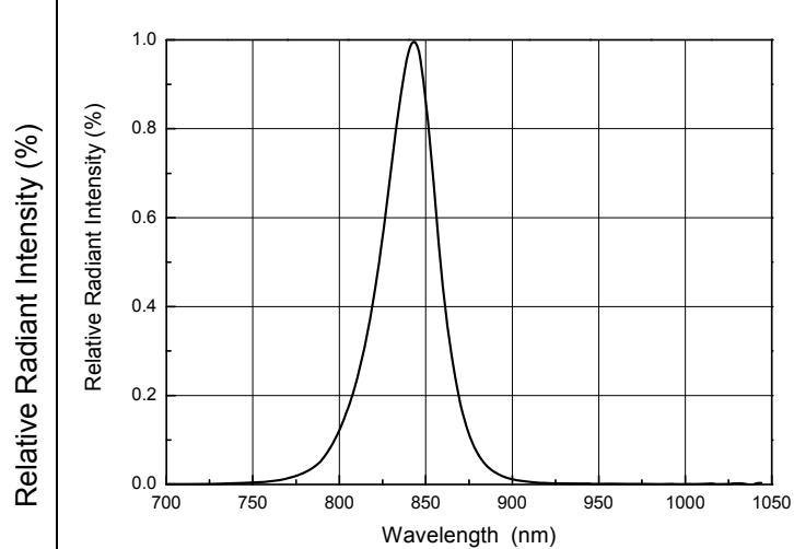
Fig.2 Spectral Distribution
