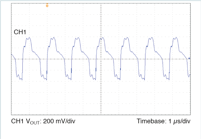
Figure 16 — Output voltage ripple, V_{IN} = 48\text{ V} , V_{OUT} = 36.0\text{ V} , C_{OUT\_EXT} = 220\ \mu\text{F} , R_{LOAD} = 4.045\ \Omega
