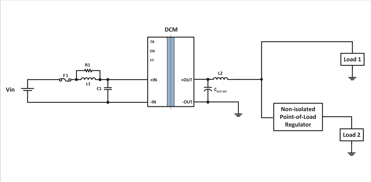
Typical Application: Single DCM3623x75H40C2y7z, to a non-isolated regulator, and direct to load
