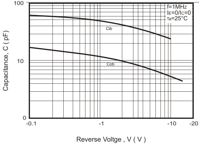
Fig. 7- C_{ob}/C_{ib} - V_{CB}/V_{EB}
