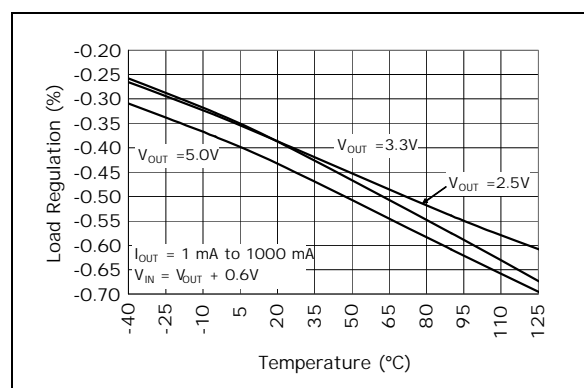
FIGURE 2-18: Load Regulation vs. Temperature ( V_{OUT} \neq 2.5V Fixed).
