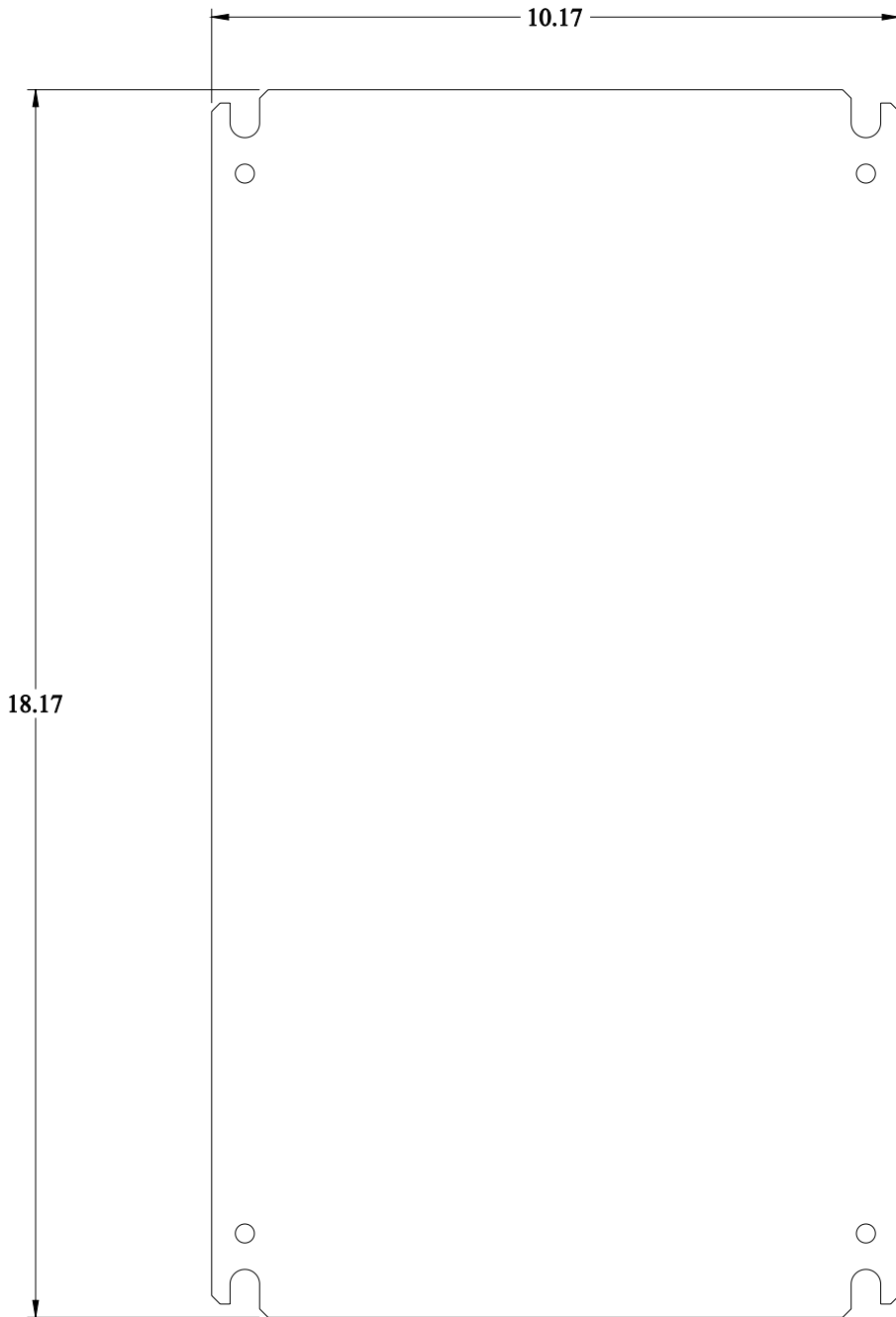
FRONT VIEW
