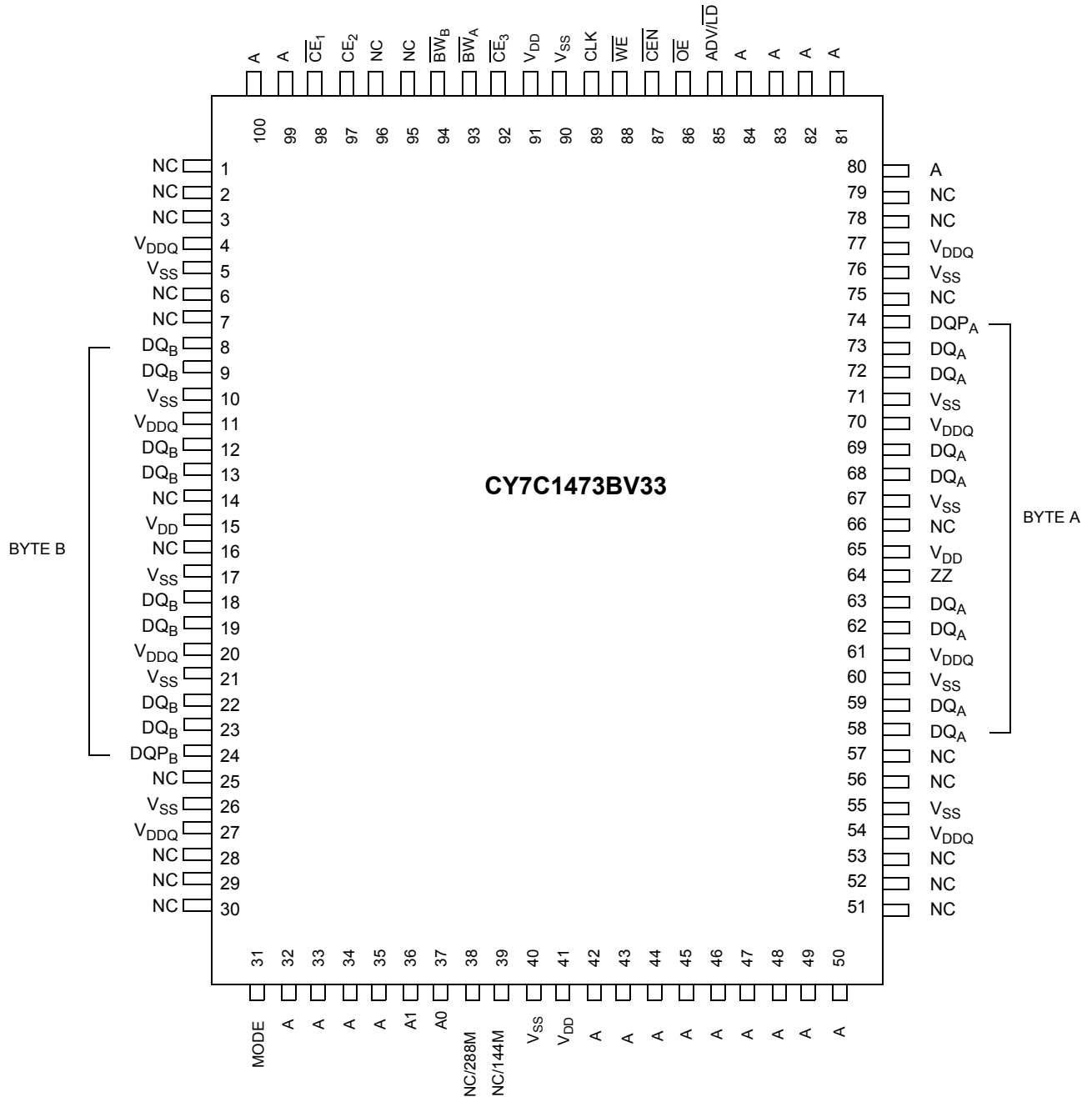
CY7C1473BV33 (4 M × 18)
