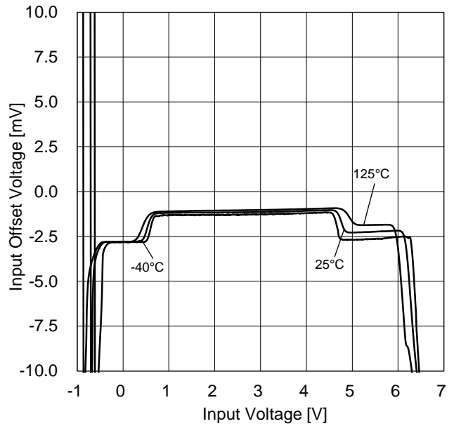
Figure 17. Input Offset Voltage vs Input Voltage ( V_{DD}=5.5V )
