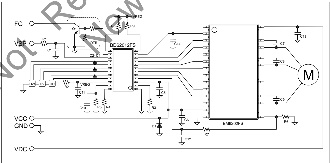
Figure 1. Application circuit example - BD62012FS & BM6202FS
