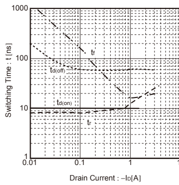
Fig.8 Switching Characteristics
