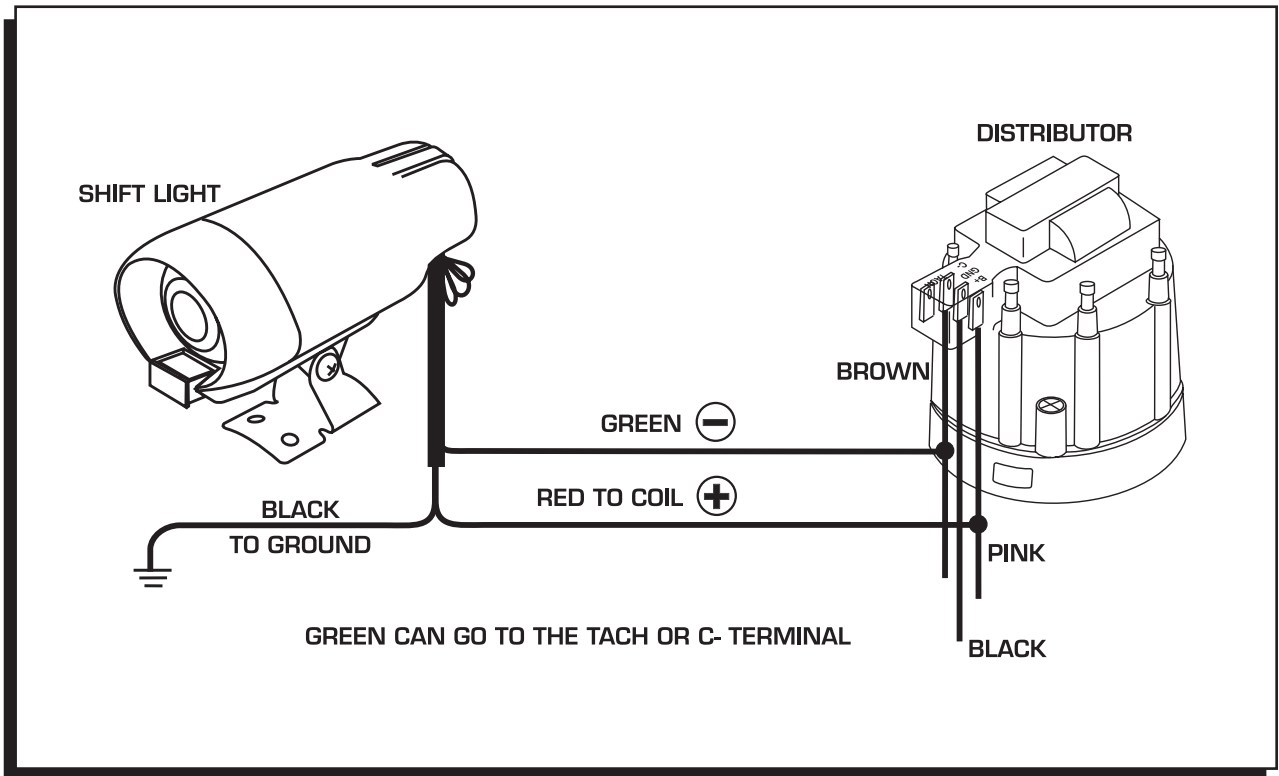
Figure 4 Wiring to a GM HEI Distributor.
