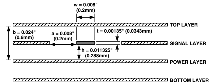
Figure 8. Cross Section of Input and Output Traces
