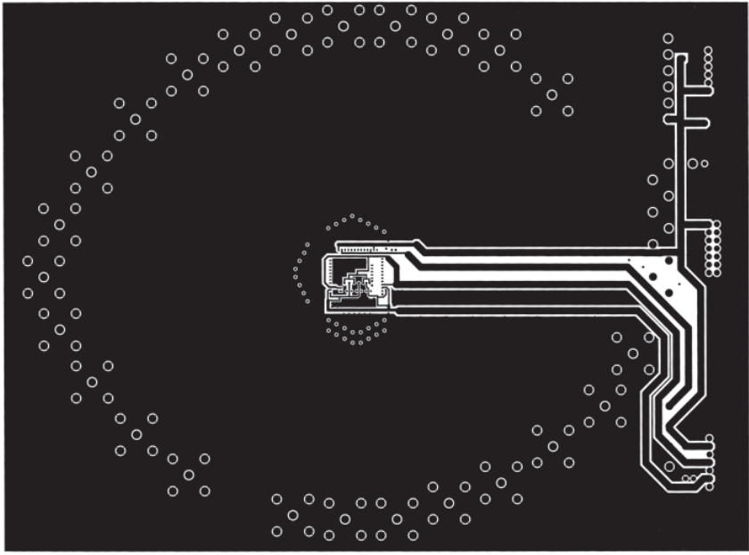
Figure 13. Board Layout (Power Plane)
