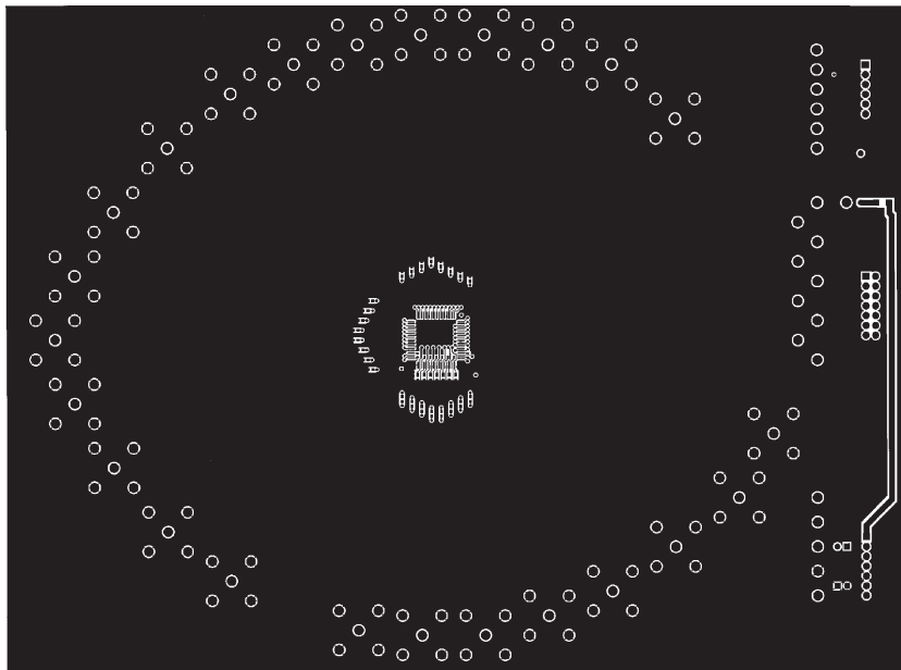
Figure 11. Board Layout (Component Side)
