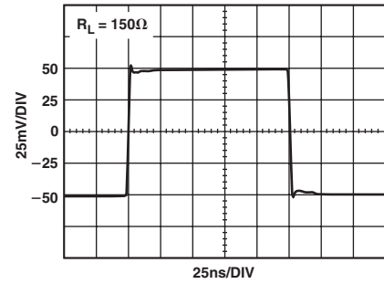
TPC 4. AD8110 Step Response, 100 mV Step
