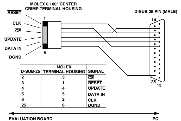
Figure 15. Evaluation Board-PC Connection Cable
