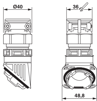
Dimensional drawing
