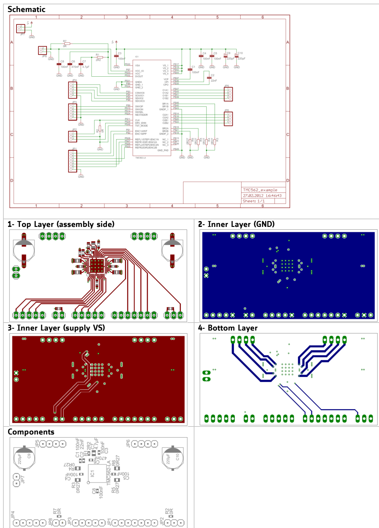
Figure 21.1 Layout example
