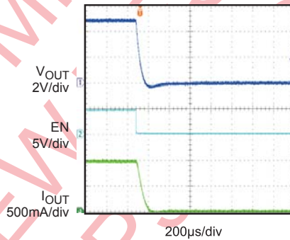
Turn Off Delay and Fall Time with 10uF Load R_{load}=5\Omega
