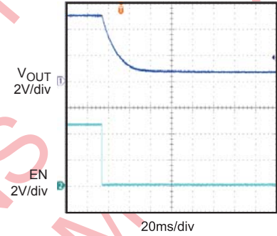
Turn Off Delay and Fall Time with 10uF Load C_{out}=10\mu F , no load
