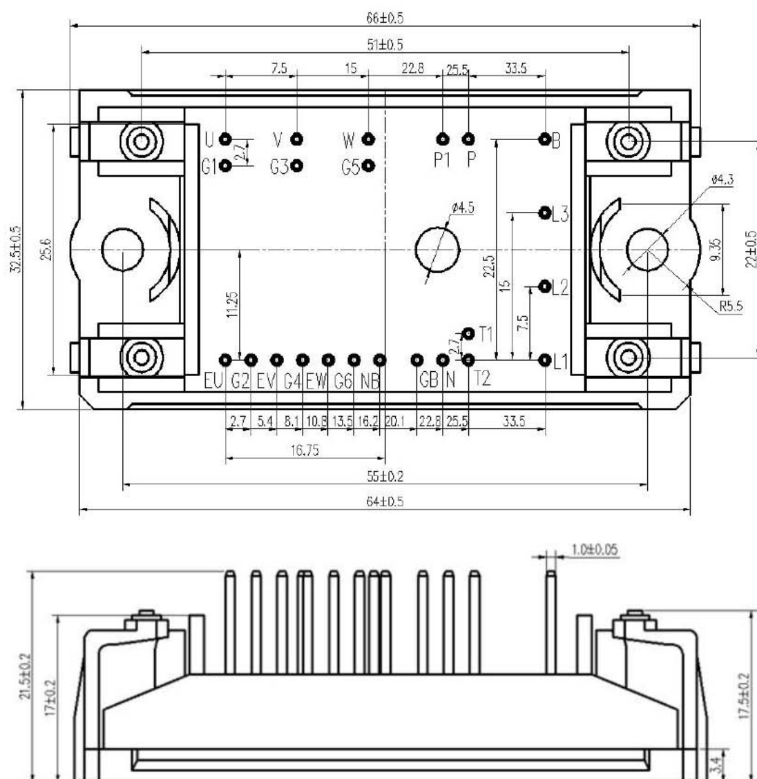
Figure12. Package Dimensions (mm)
