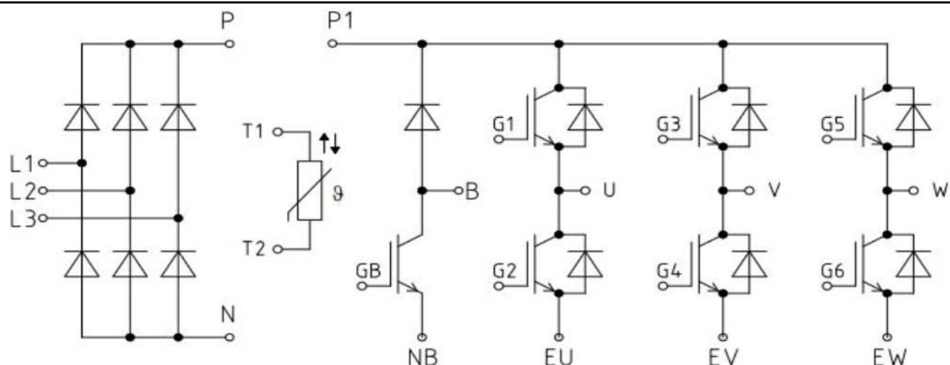
Figure11. Circuit Diagram
