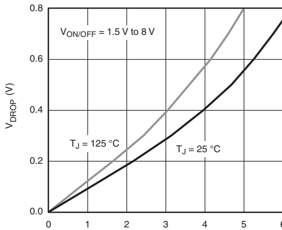
V_{DROP} vs. I_L at V_{IN} = 1.8 V
