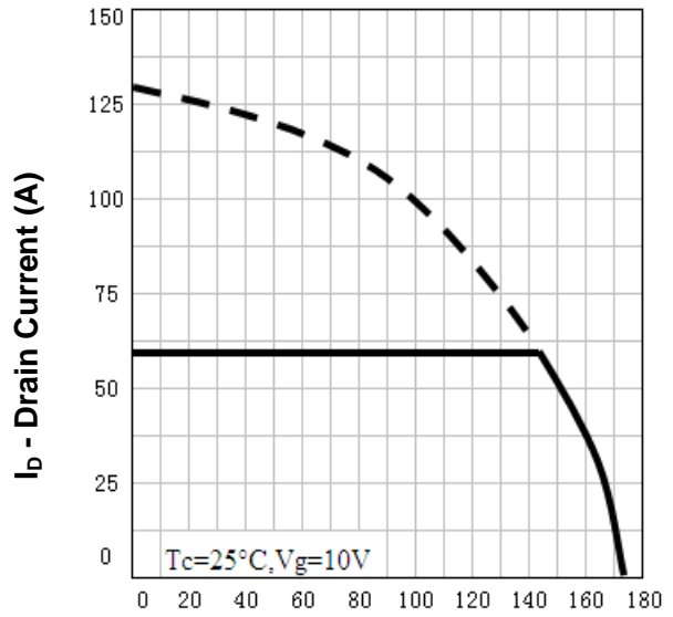
Drain Current
