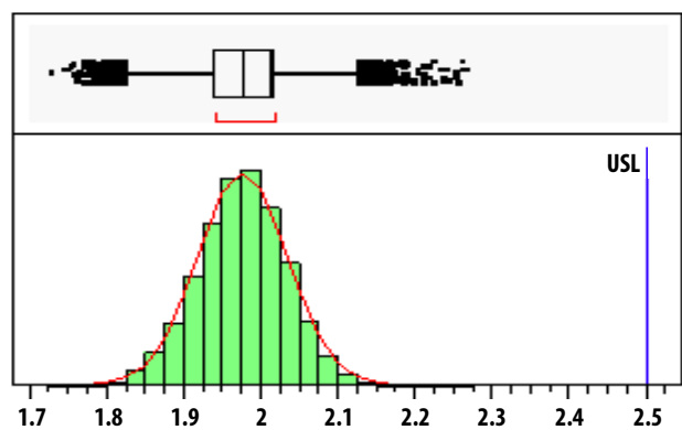
NF @ 6GHz, Mean=2dB, USL=2.5dB
