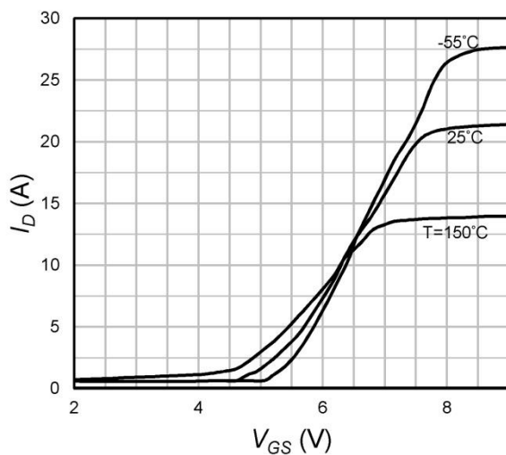
Fig.5 Transfer Characteristics
