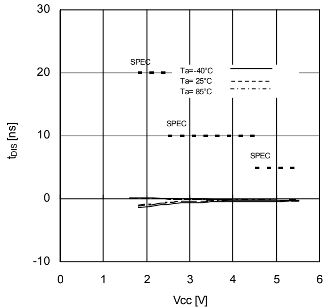
Figure 25. SI Setup Time vs Supply Voltage
