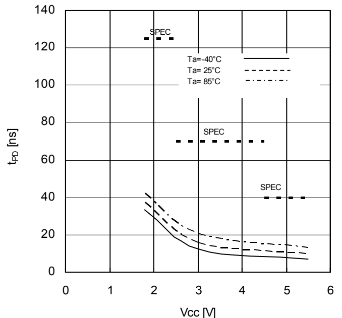
Figure 27. Data Output Delay Time vs Supply Voltage
