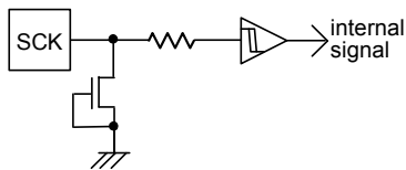
Figure 53. SCK input equivalent circuit
