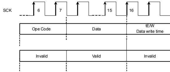
Figure 42. WPB valid timing (At inputting WRSR command)
