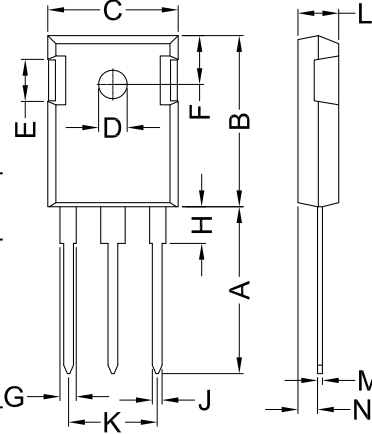
Dimensions TO-247AD
