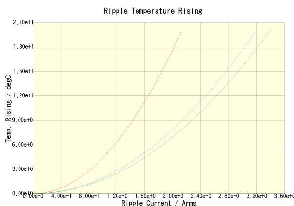
C3216X7R2A105K160AA(100kHz) C3216X7R2A105K160AA(500kHz) C3216X7R2A105K160AA(1MHz)
