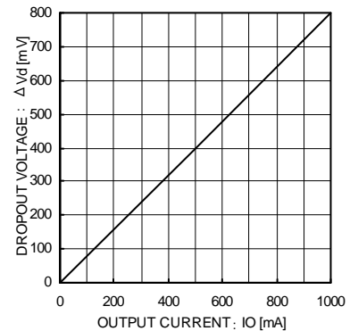
Fig.6 Dropout Voltage (Vcc=Vo x 0.95V) (Io=0mA→1000mA)
