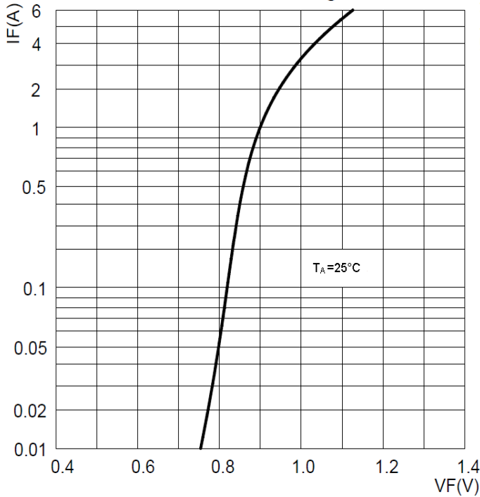
FIG3: Forward Voltage
