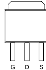
TO-251S(JB)
