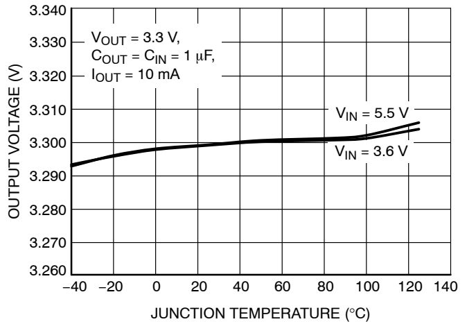
Figure 18. Output Voltage vs. Temperature, V_{OUT} = 3.3 V
