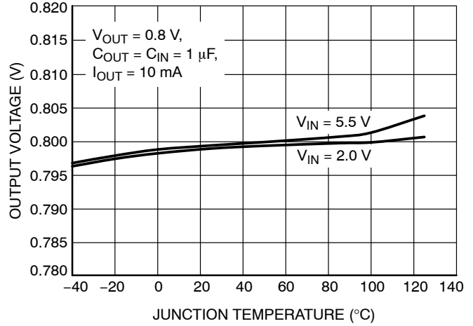
Figure 16. Output Voltage vs. Temperature, V_{OUT} = 0.8 V
