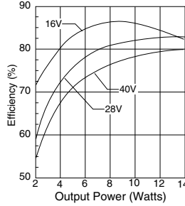
HR121-2812 Efficiency FIGURE 3
