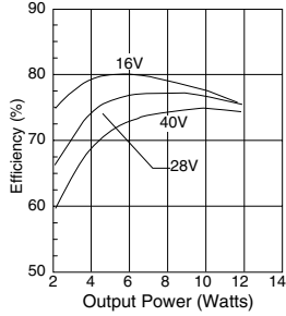
HR121-2805 Efficiency FIGURE 2
