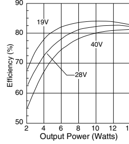
HR122-2815 Efficiency
