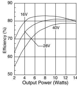
HR122-2812 Efficiency
