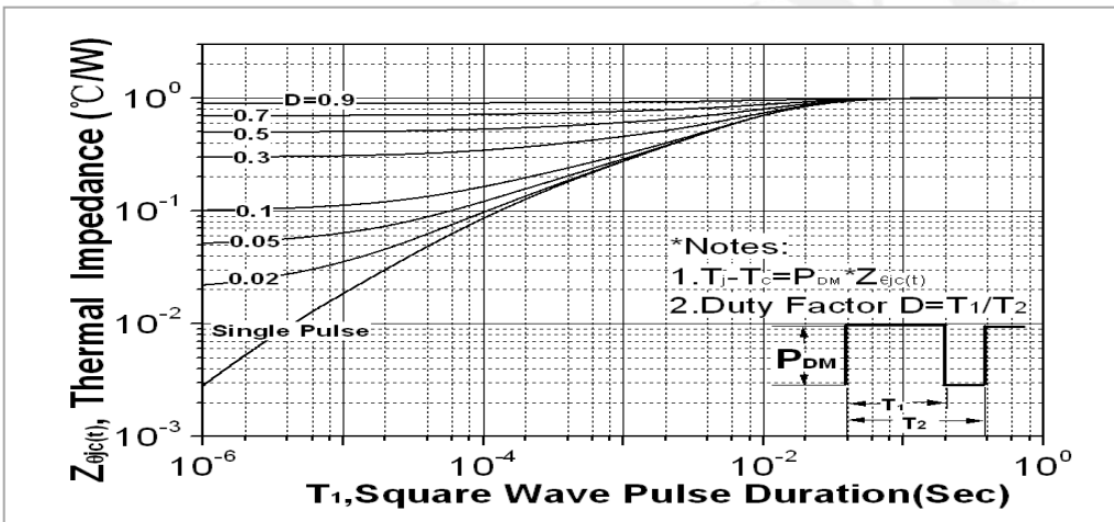
Fig. 14. Transient thermal response curve(TO-220)
