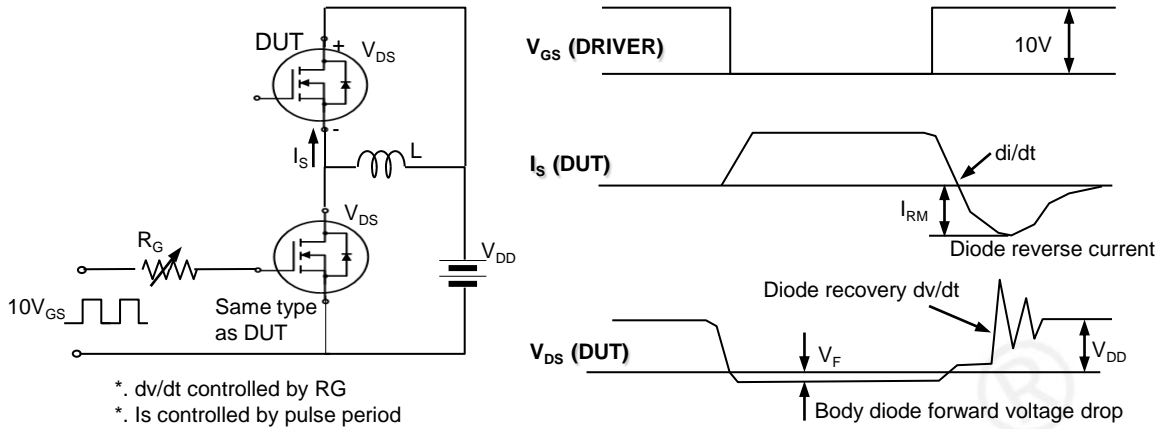
Fig. 18. Peak diode recovery dv/dt test circuit & waveform
