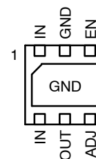
NCP691, NCP692 – DFN6
