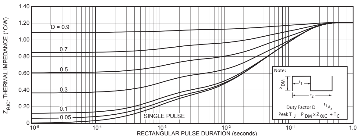
FIGURE 22, MAXIMUM EFFECTIVE TRANSIENT THERMAL IMPEDANCE, JUNCTION-TO-CASE vs. PULSE DURATION
