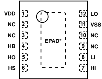
ISL2110AR4Z, ISL2111AR4Z (12 LD 4x4 DFN) TOP VIEW
