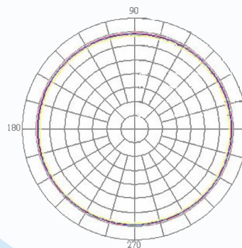
H Plane - Azimuth @700 MHz
