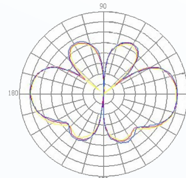
E Plane - Vertical @700 MHz
