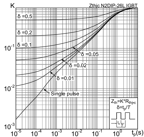
Figure 16. Thermal impedance
