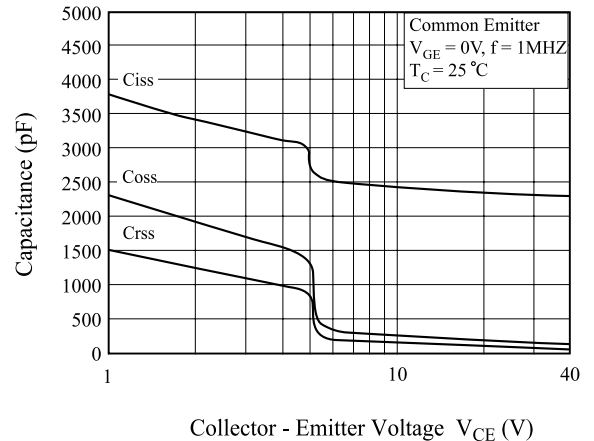
Fig 6. Capacitance Characteristics
