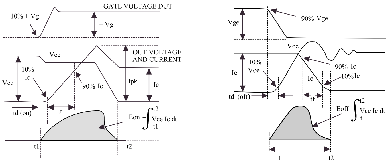
Fig 18. Definition Switching Time & Loss
