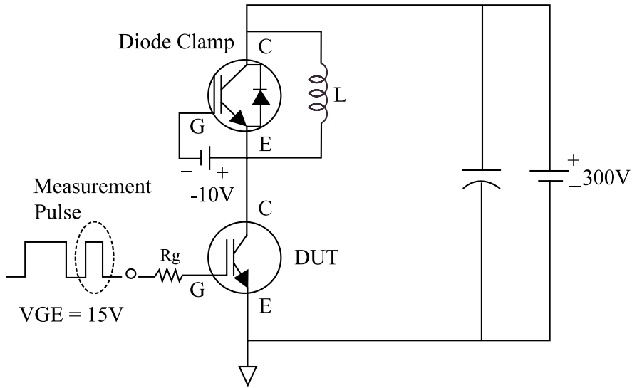
Fig 18. Definition Switching Time & Loss
