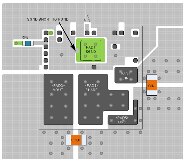
FIGURE 43. RECOMMENDED LAYOUT
