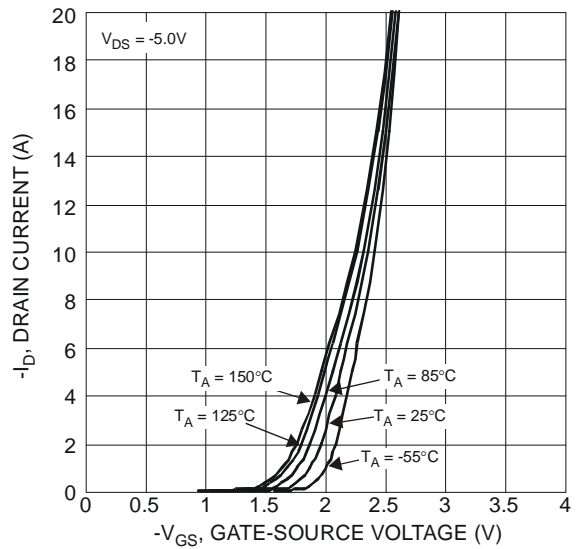
Figure 12 Typical Transfer Characteristics
