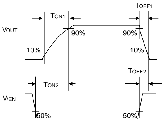
Figure 2. Timing diagram (BD2061AFJ)
