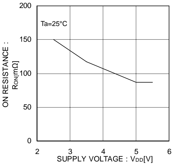
Figure 12. ON resistance
