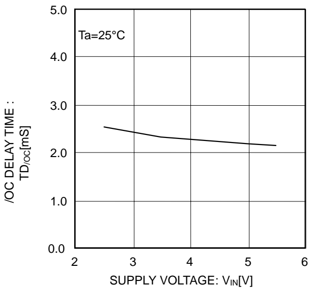
Figure 14. /OC output delay time
