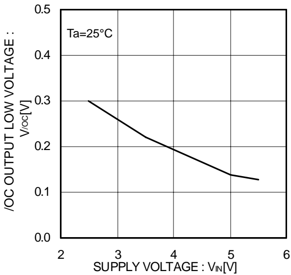
Figure 10. /OC output LOW voltage
