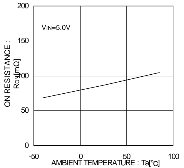
Figure 13. ON resistance
