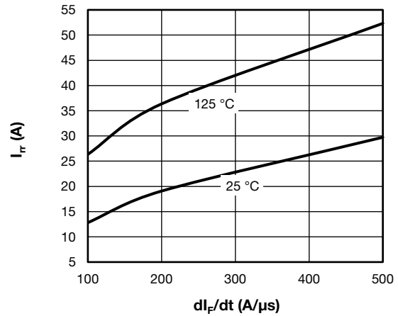
Fig. 8 - Typical Reverse Recovery Current vs. di F /dt
