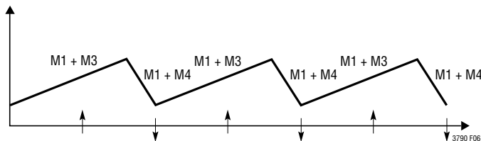
Figure 6. Boost Operation ( V_{IN} < V_{OUT} )
