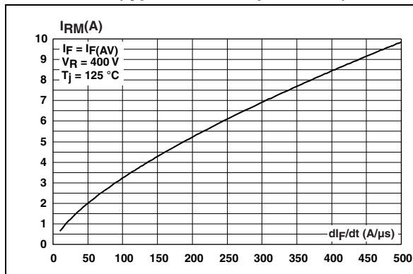
Figure 5. Peak reverse recovery current versus dl_F/dt (typical values, per diode)
